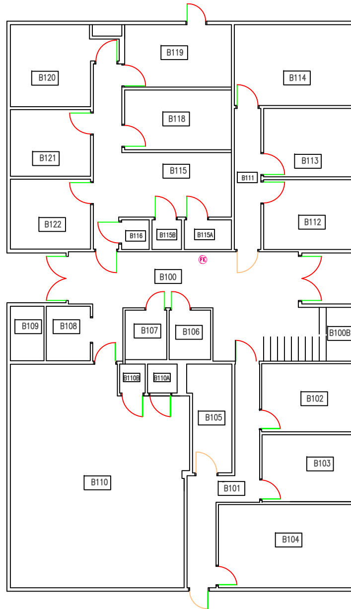
BUILDING B FIRST FLOOR
