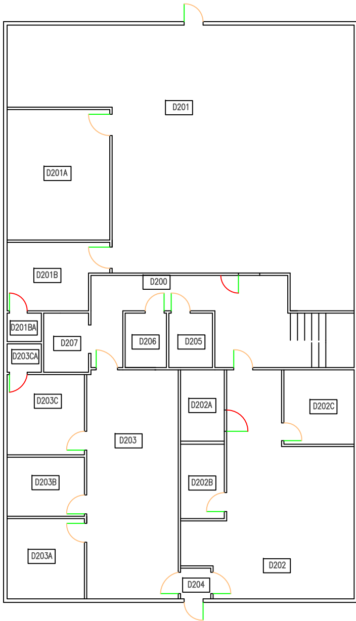
BUILDING D SECOND FLOOR
